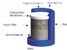
Typical VRLA Catalyst
